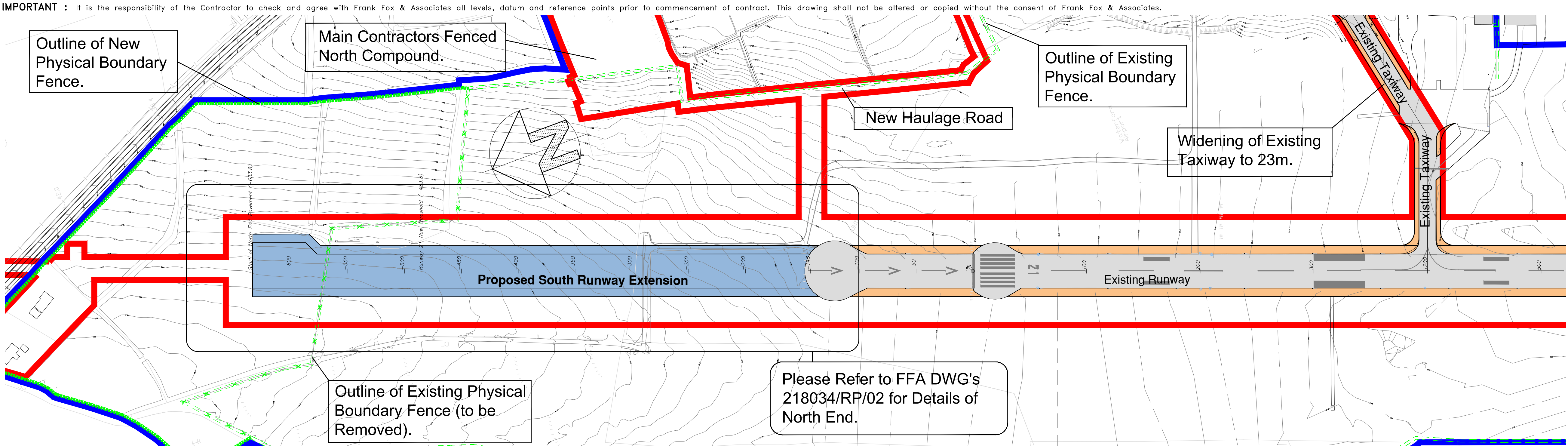
GENERAL ARRANGEMENT LAYOUT NORTH END
