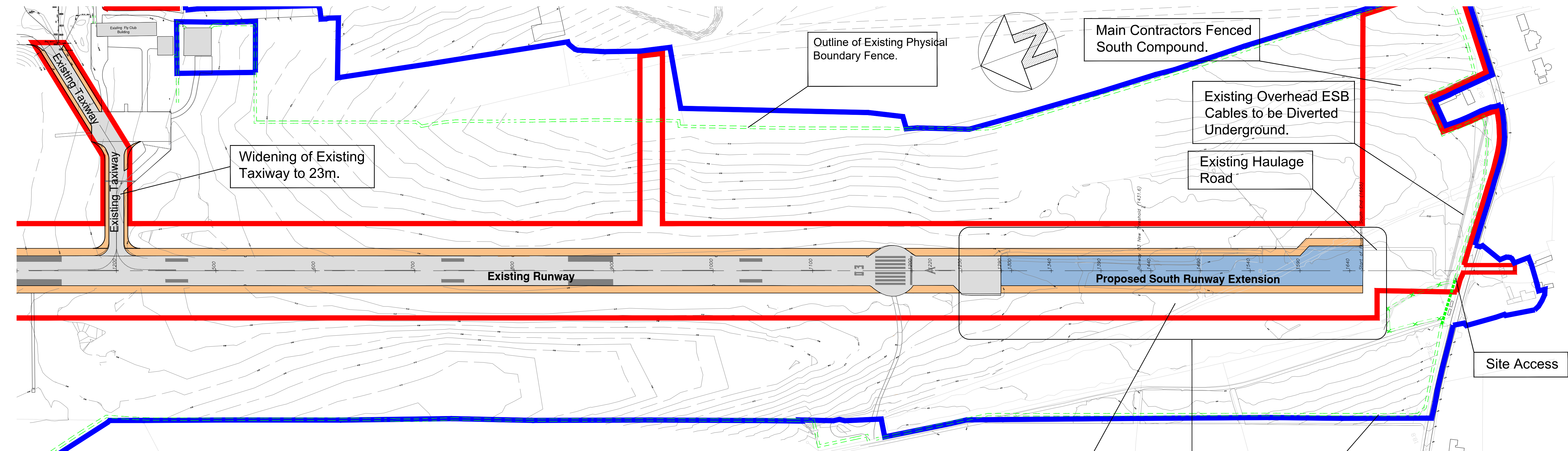
GENERAL ARRANGEMENT LAYOUT SOUTH END
